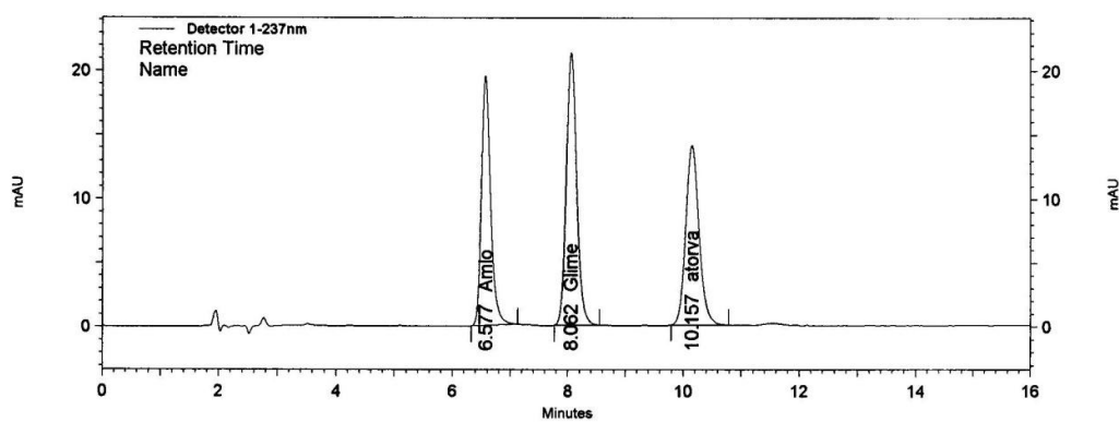
Figure 3.27. Chromatogram of amlodipine, glimepiride, and atorvastatin assayed in 5% increase of ACN.
